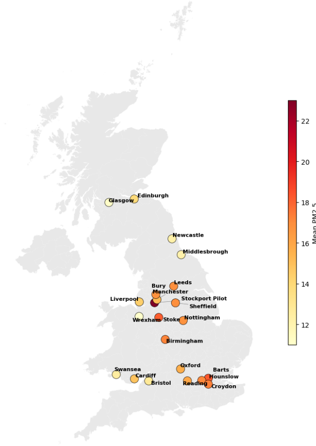
Figure 3: Mean PM2.5 across UK Biobank assessment centers, averaged over all assessment days.
