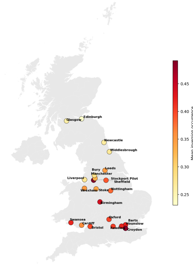
Figure 2: Inversion occurrence across UK Biobank assessment centers, averaged over all assessment days.
